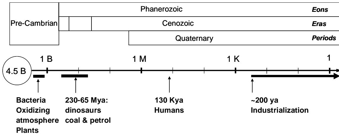
Figure 1: Geological time scales. (Notation: ya= years ago, K=10 3 , M=10 6 , B=10 9 )
