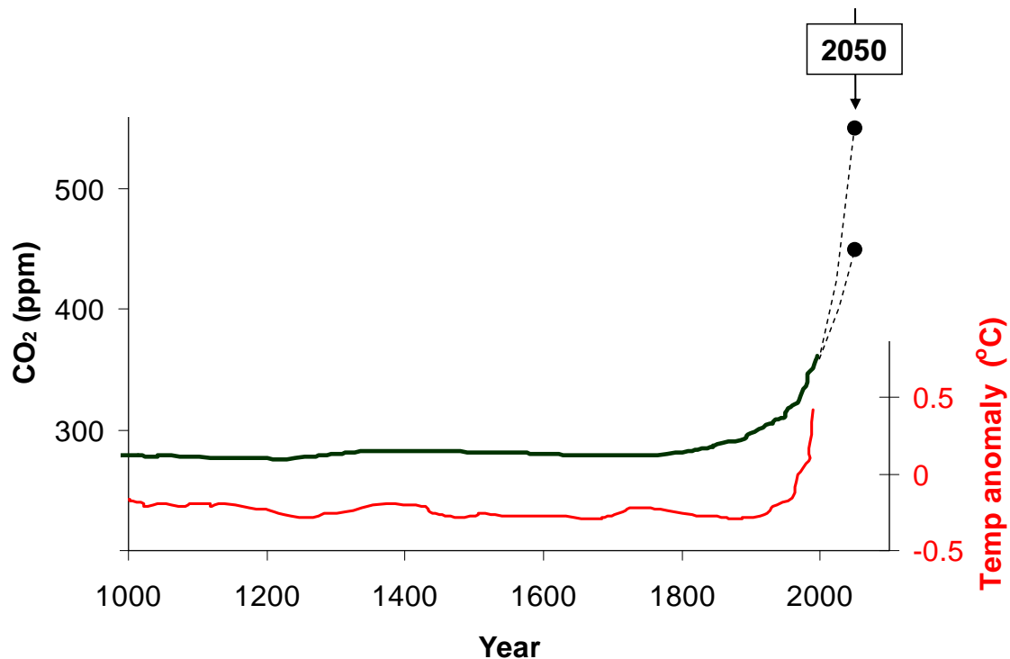
Figure 7: Carbon emission and global warming (highly filtered trend – original data from Mann and Jones 2003; see IPCC 2007)
